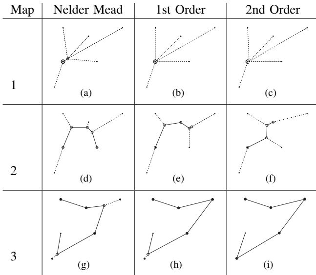
Fig. 3. Rendezvous solutions discovered. Tanker is at the solid spot on figure (a), other points show workers. Circles denote meeting places. Tanker route is shown with solid lines, workers routes are shown with dashed lines.
